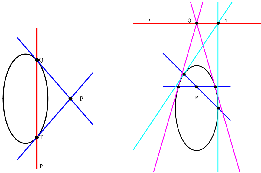
Figure 15: Polars (red) of a point P outside or inside an ellipse.
