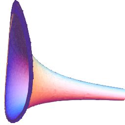
Figure 20: Hyperbolic inverse of a pseudosphere.
