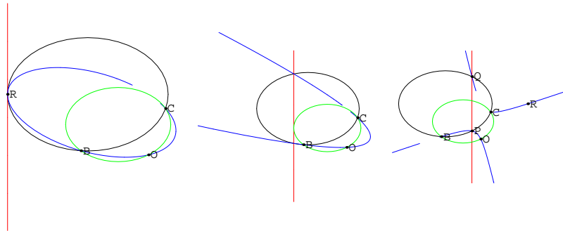
Figure 17: Inversion of three parallel straight lines
