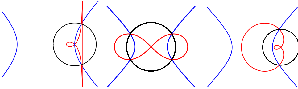
Figure 8: A hyperbola with its inverses with respect to circles centered in one of its vertices (left), in its center (middle) and in one of its foci (right)
