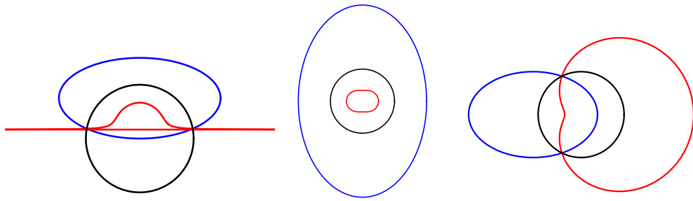
Figure 7: An ellipse with its inverses with respect to circles centered in one of its vertices (left), in the center (middle) and in one of its foci (right)
