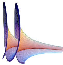
Figure 21: Hyperbolic inverse of a Dini's surface.
