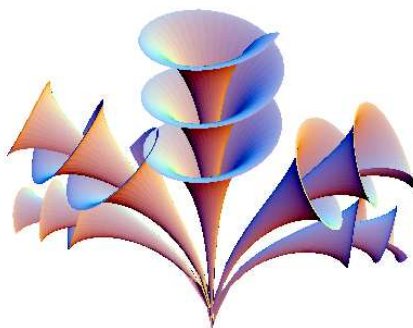
Figure 5: A Dini bouquet
