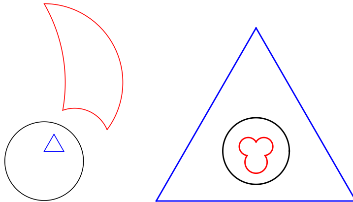
Figure 9: Inverses of a triangle contained in (left) and containing (right) the circle of inversion.
