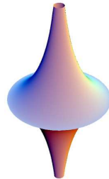
Figure 4: Pseudosphere
